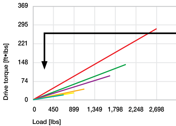
Diagram 01: Required drive torque versus applied load
